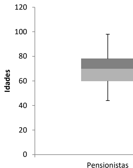
BOXPLOT PENSIONISTAS
